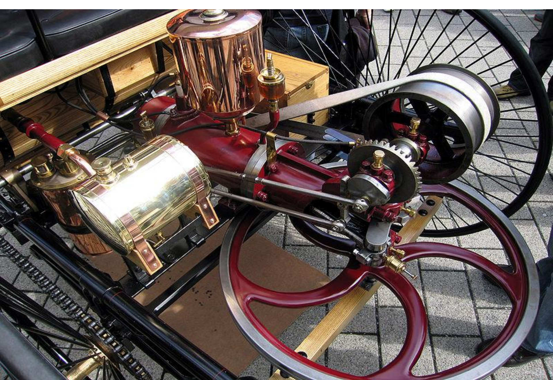
Engine of the Benz Patent Motorwagen
