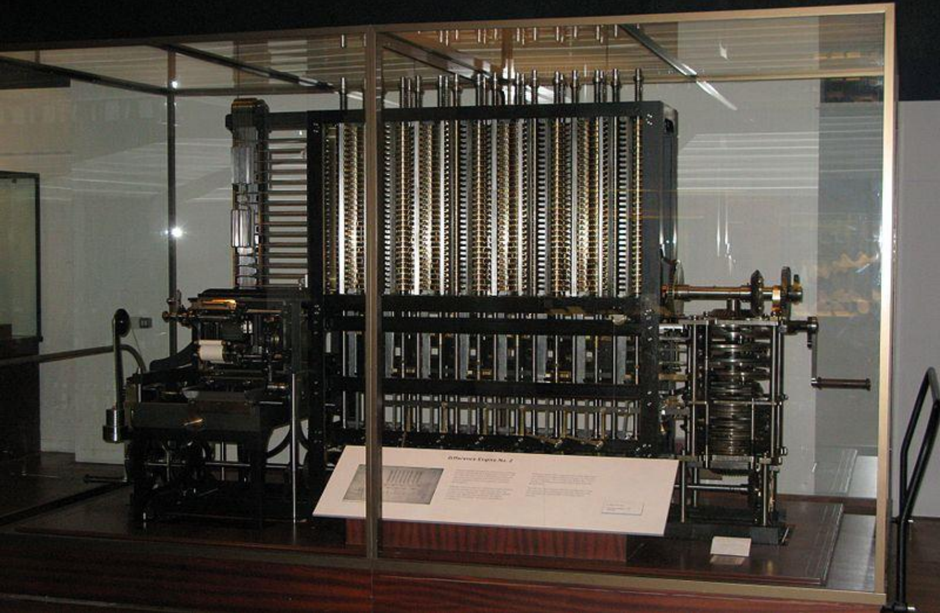
The Science Museum's Difference Engine No. 2, built from Babbage's design
